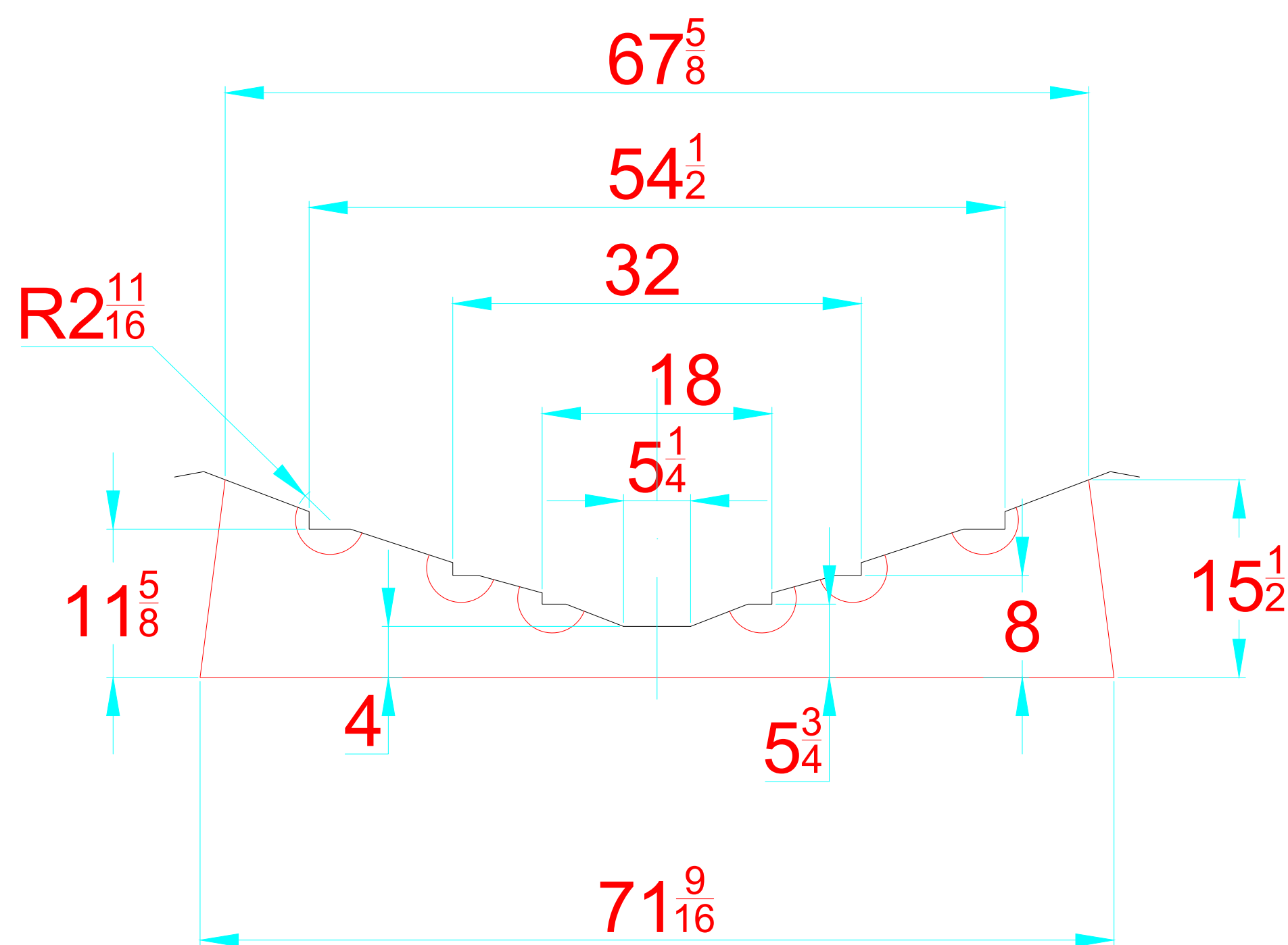
TRANSVERSAL SECTION "A" SECCION TRANSVERSAL "A"
