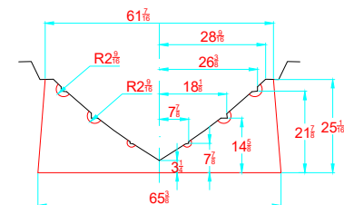
TRANSVERSAL SECTION "C" SECCION TRANSVERSAL "C"
