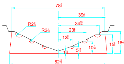
TRANSVERSAL SECTION "A" SECCION TRANSVERSAL "A"
