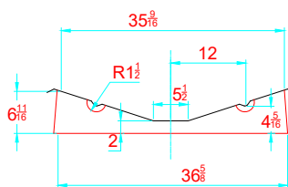
TRANSVERSAL SECTION "A" SECCION TRANSVERSAL "A"
