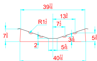
TRANSVERSAL SECTION "A" SECCION TRANSVERSAL "A"
