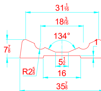
TRANSVERSAL SECTION "A" SECCION TRANSVERSAL "A"
