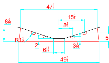
TRANSVERSAL SECTION "A" SECCION TRANSVERSAL "A"
