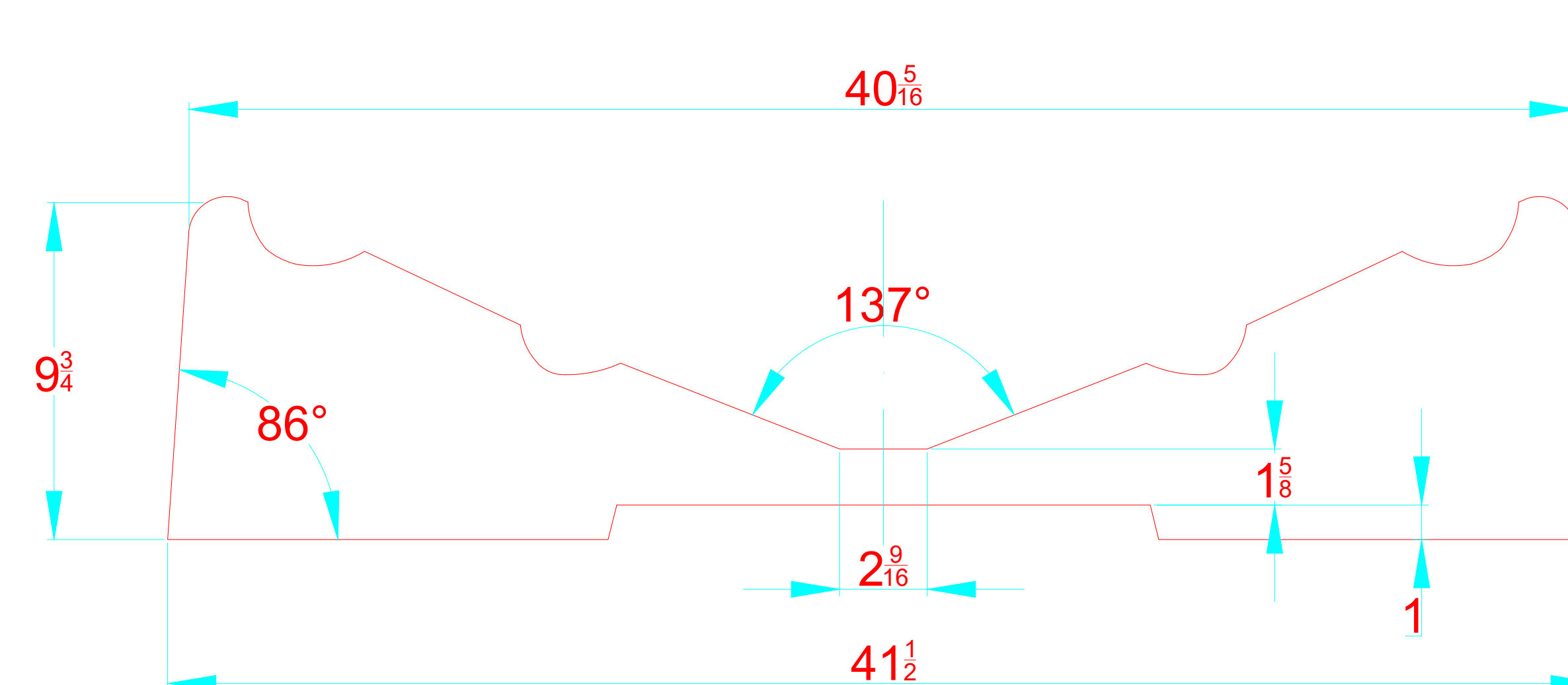
TRANSVERSAL SECTION "A" SECCION TRANSVERSAL "A"
