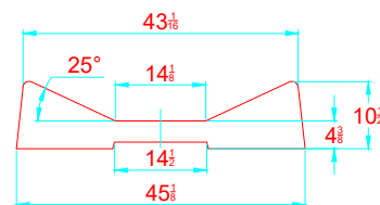
TRANSVERSAL SECTION "A" SECCION TRANSVERSAL "A"
