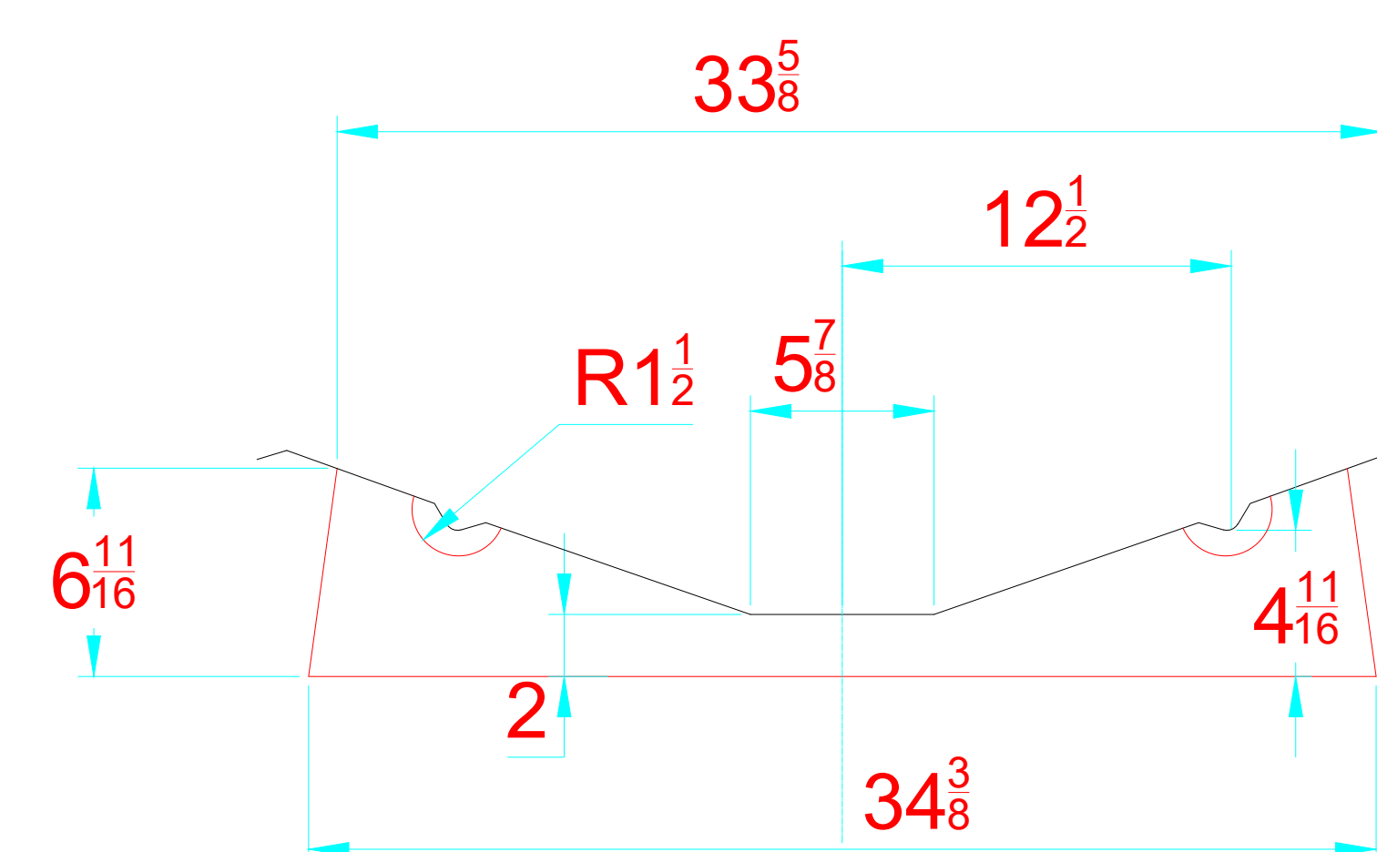
TRANSVERSAL SECTION "A" SECCION TRANSVERSAL "A"
