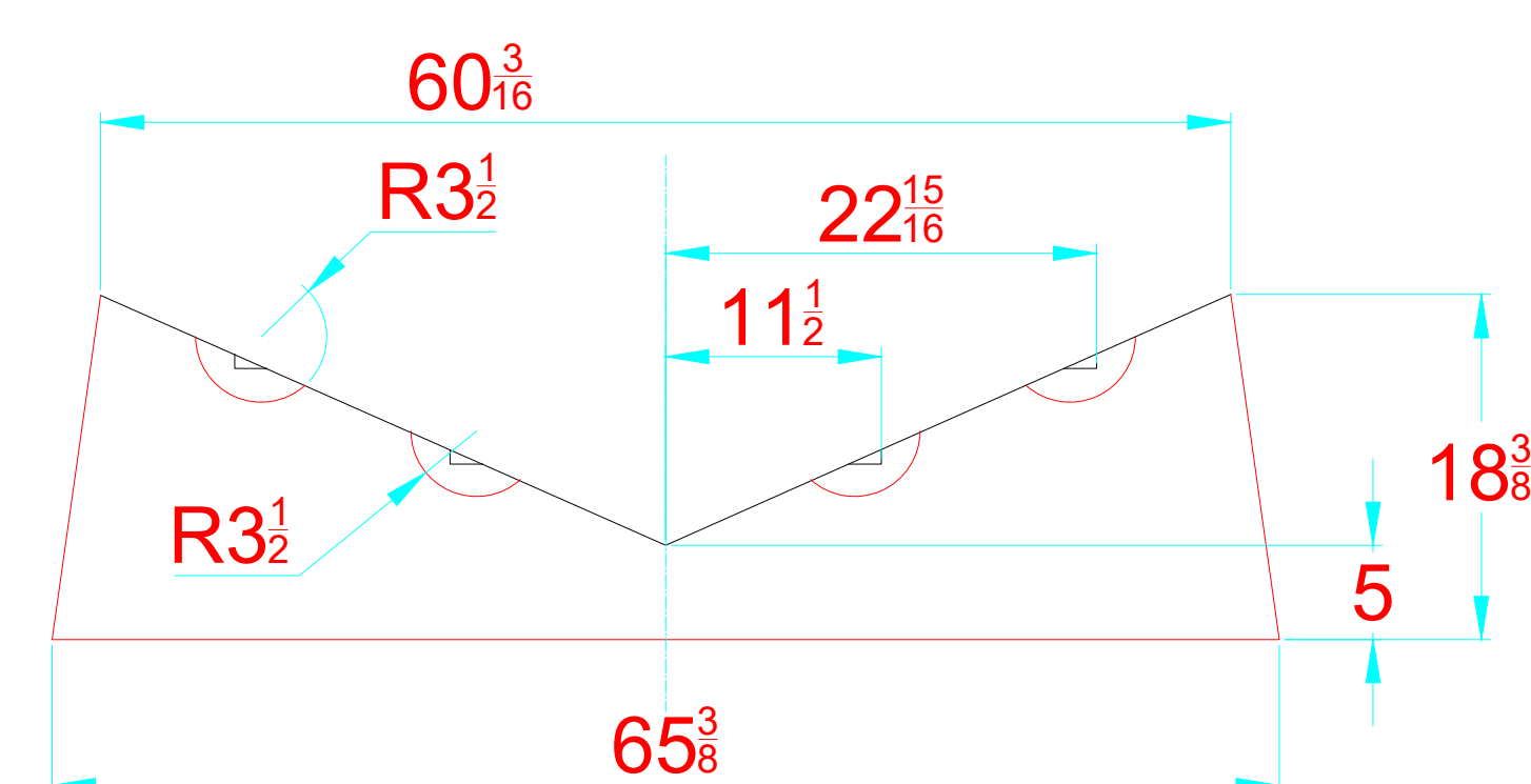
TRANSVERSAL SECTION "A" SECCION TRANSVERSAL "A"
