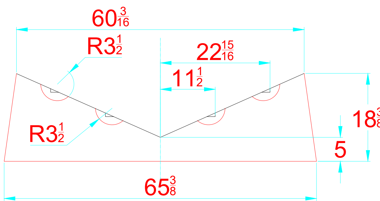
TRANSVERSAL SECTION "A" SECCION TRANSVERSAL "A"
