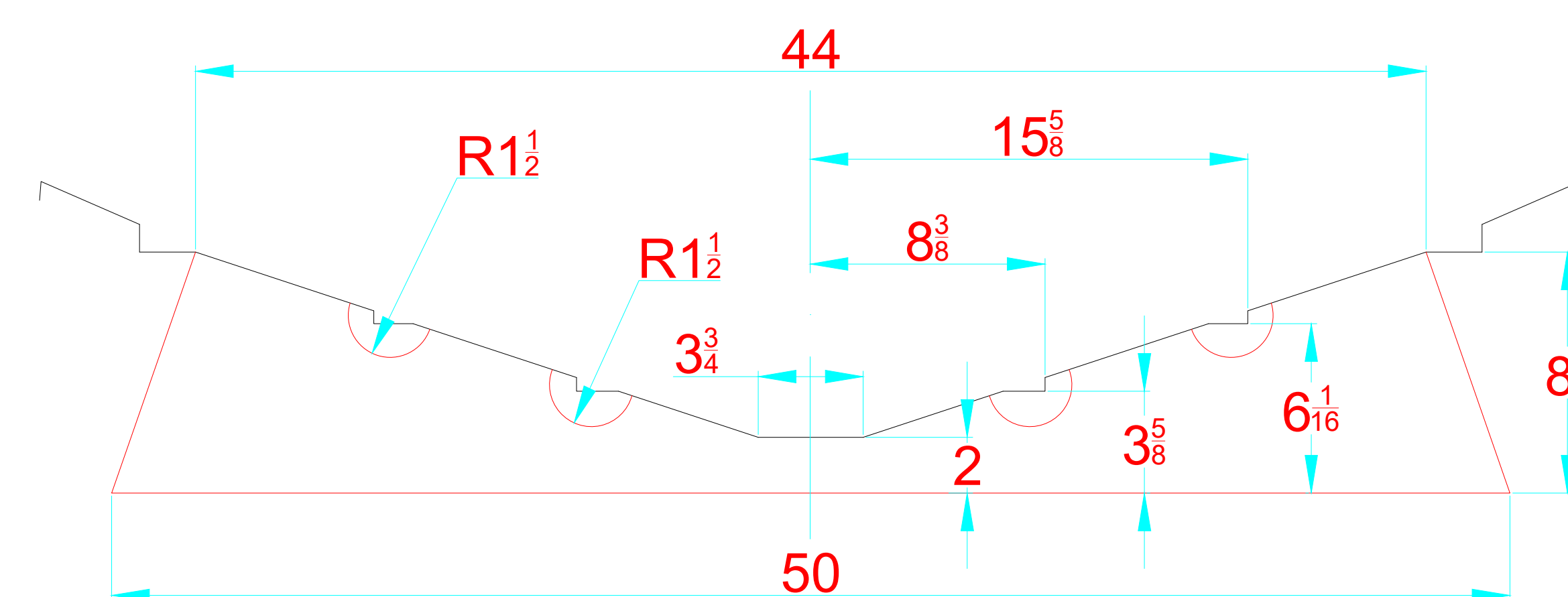
TRANSVERSAL SECTION "A" SECCION TRANSVERSAL "A"
