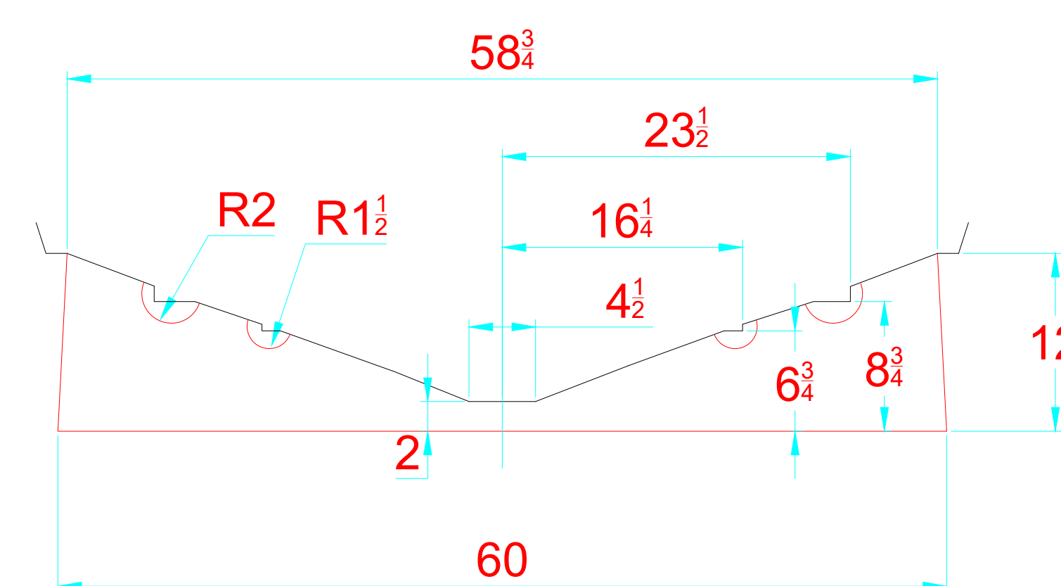
TRANSVERSAL SECTION "A" SECCION TRANSVERSAL "A"
