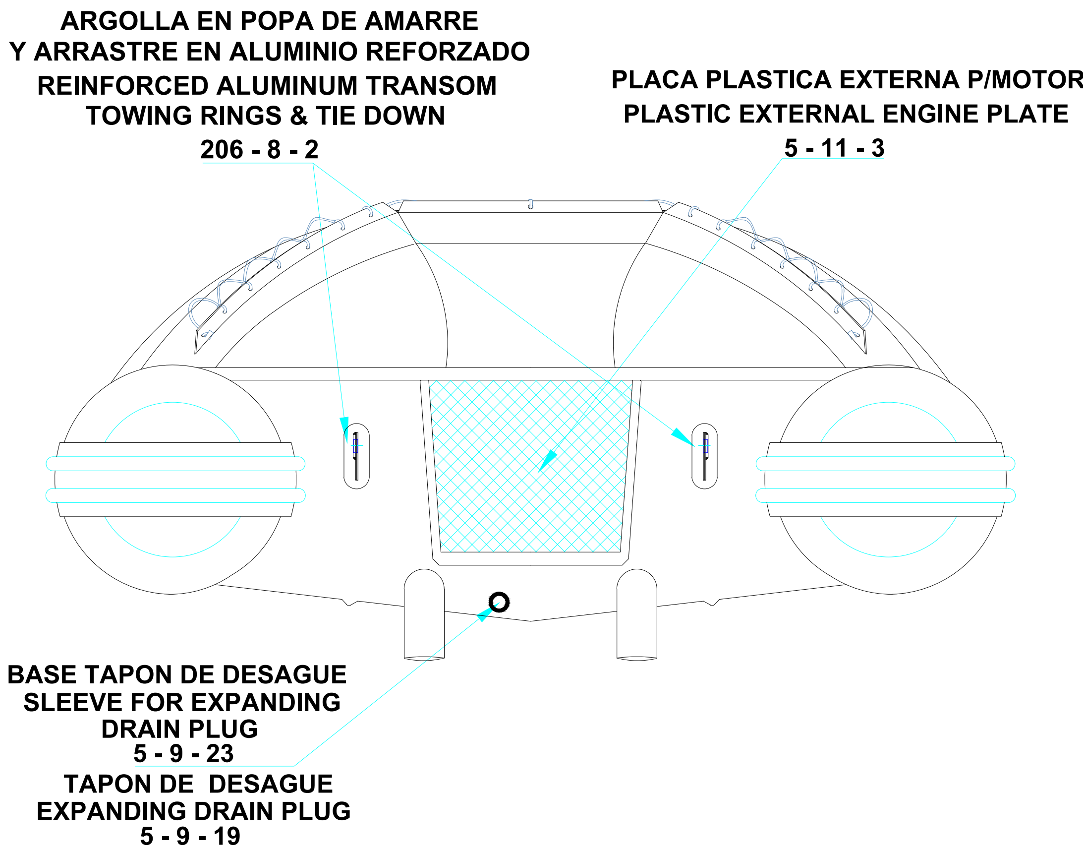
AFT VIEW VISTA TRASERA
