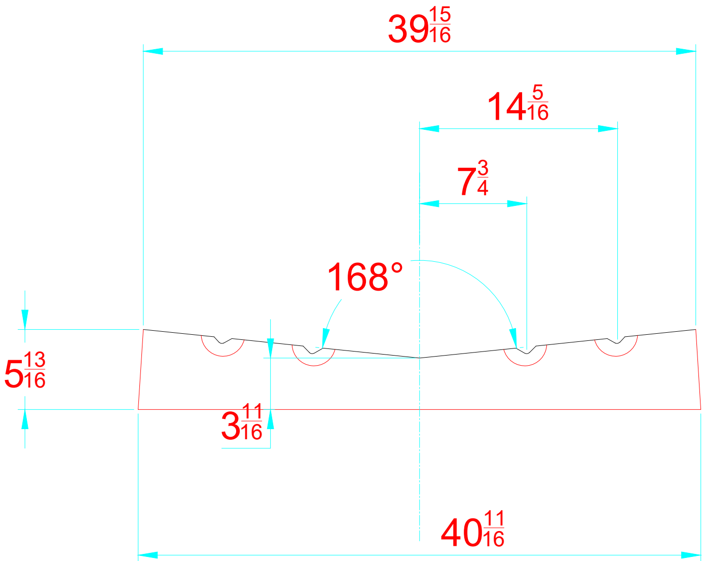
TRANSVERSAL SECTION "A" SECCION TRANSVERSAL "A"
