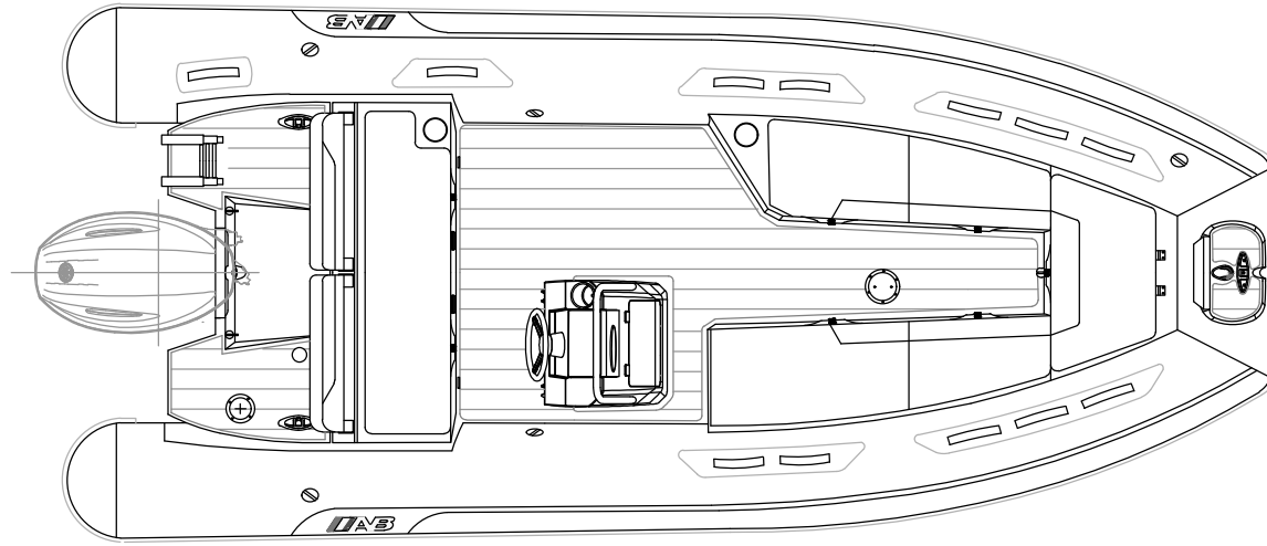
PLANT VIEW
